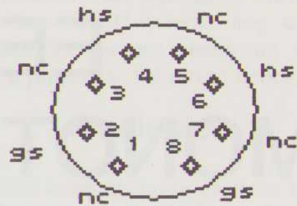
5U4G
